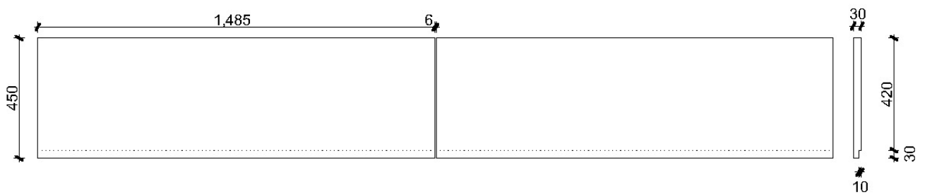
1485x450x30mm without rebated course line
