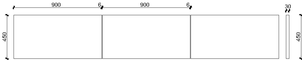
900x450x30mm without rebated course line
