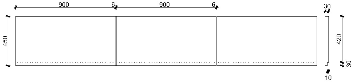
900x450x30mm with rebated course line
