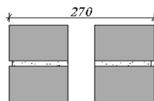
double brick cavity wall
